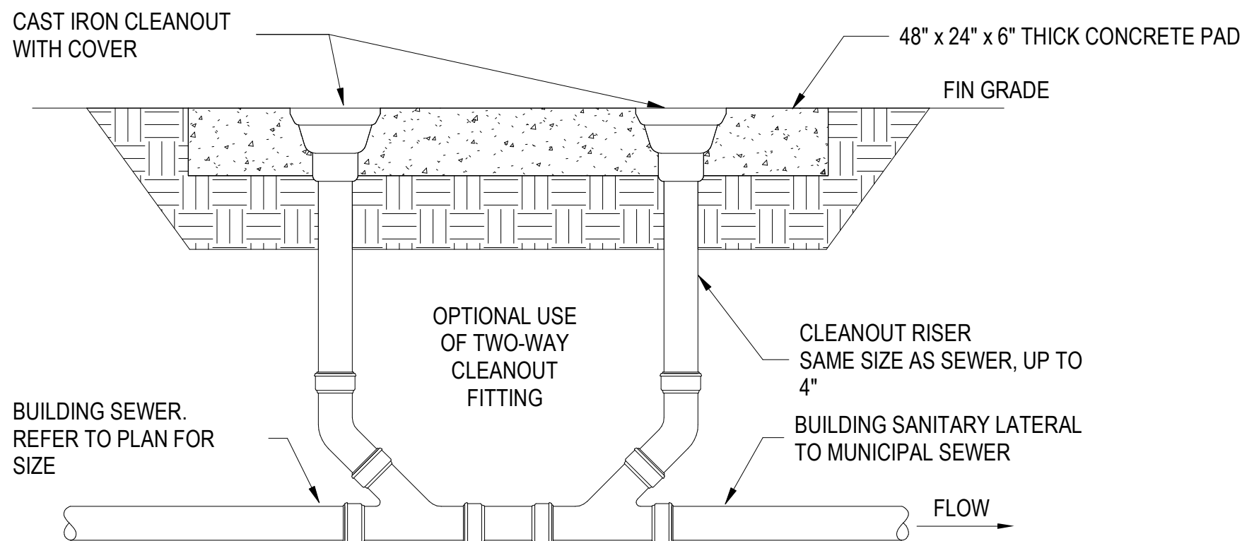
2 TWO-WAY CLEANOUT SCALE:NTS
