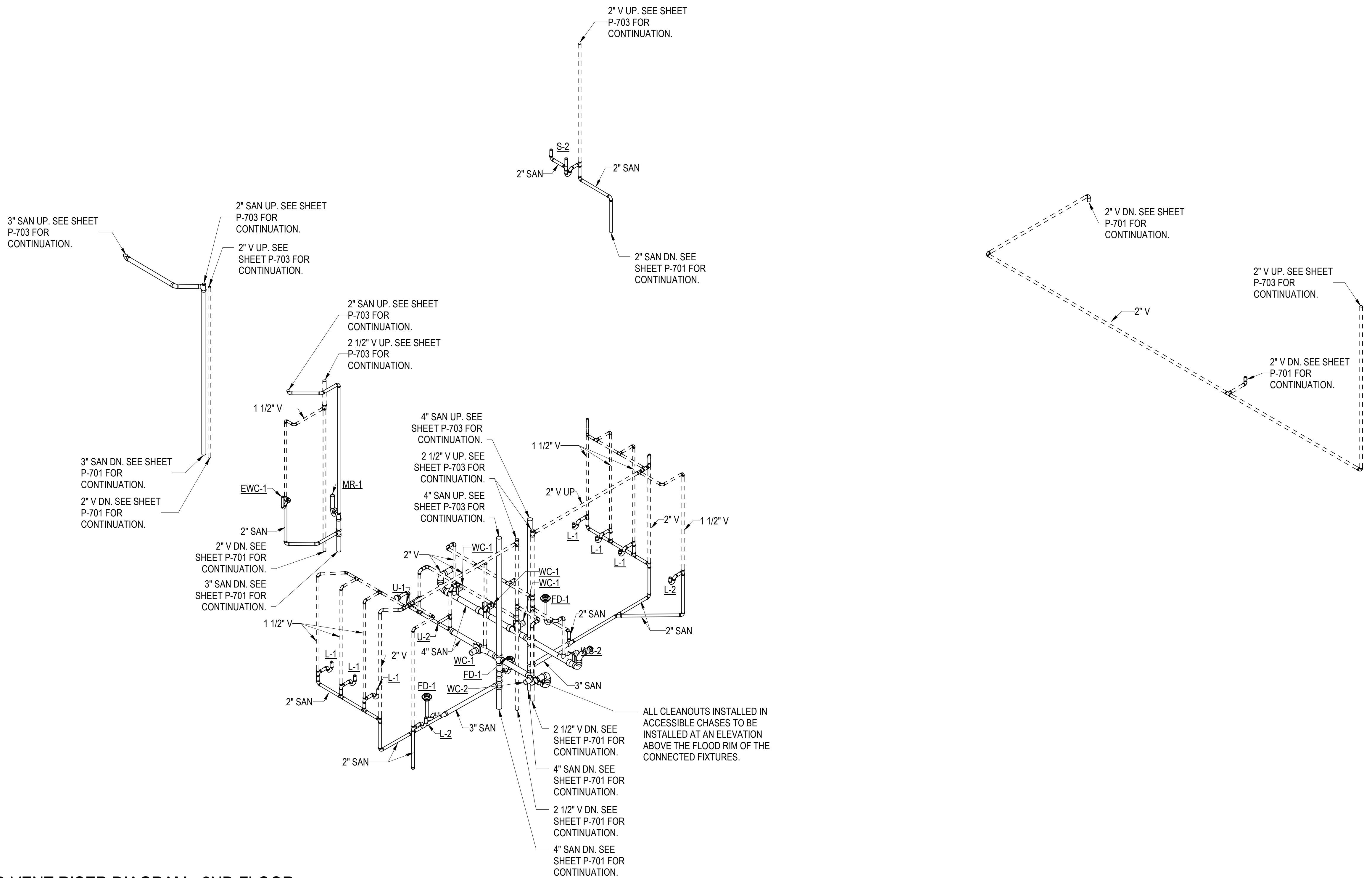
1 WASTE AND VENT RISER DIAGRAM - 2ND FLOOR SCALE: NTS
