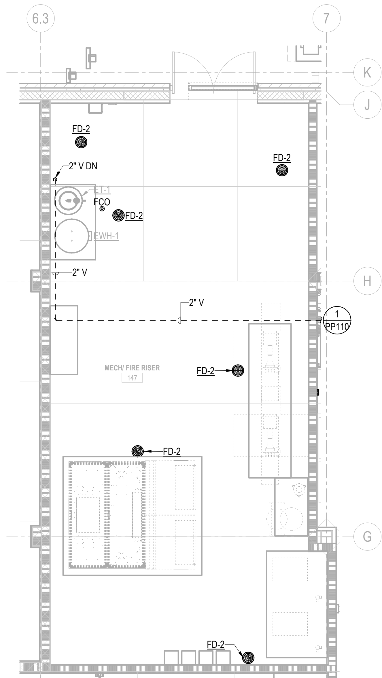
1 ENLARGED PLUMBING PLAN - MECH ROOM - WASTE & VENT SCALE: 1/4" = 1'-0"
