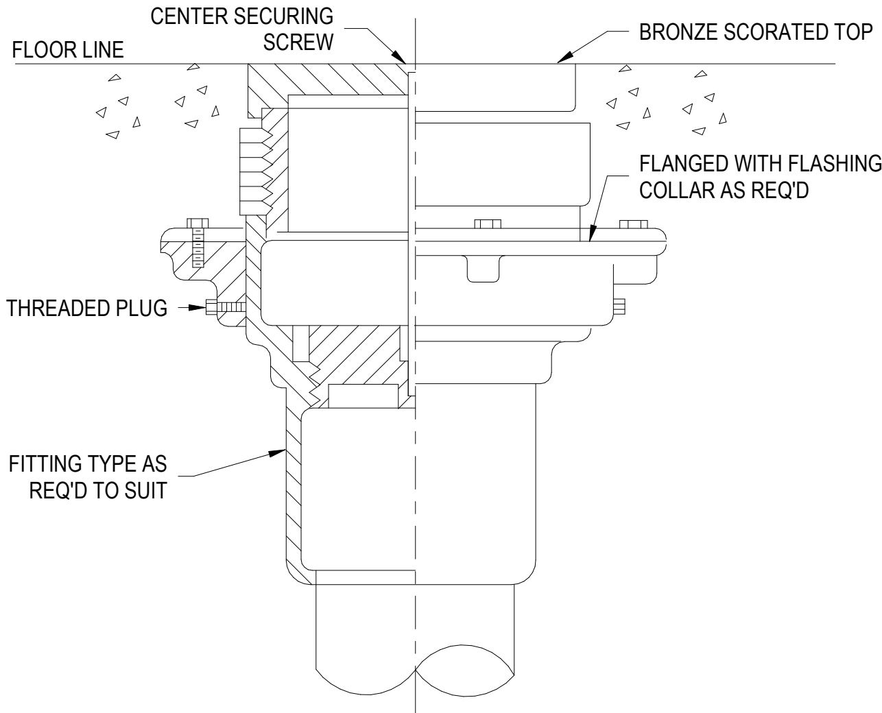
3 FLOOR CLEANOUT - BODY SCALE:NTS
