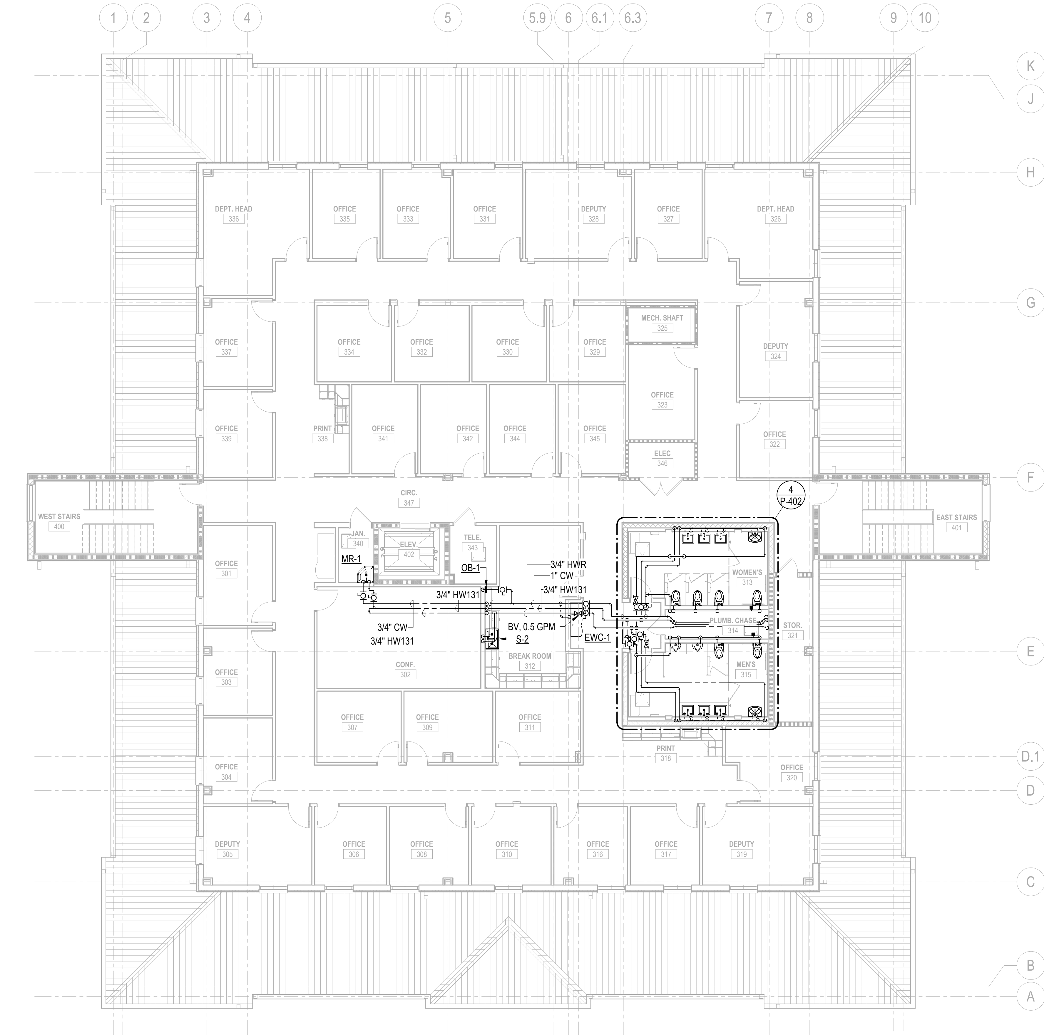
PLUMBING - WATER - 3RD FLOOR PLAN SCALE: 1/8" = 1'-0"
