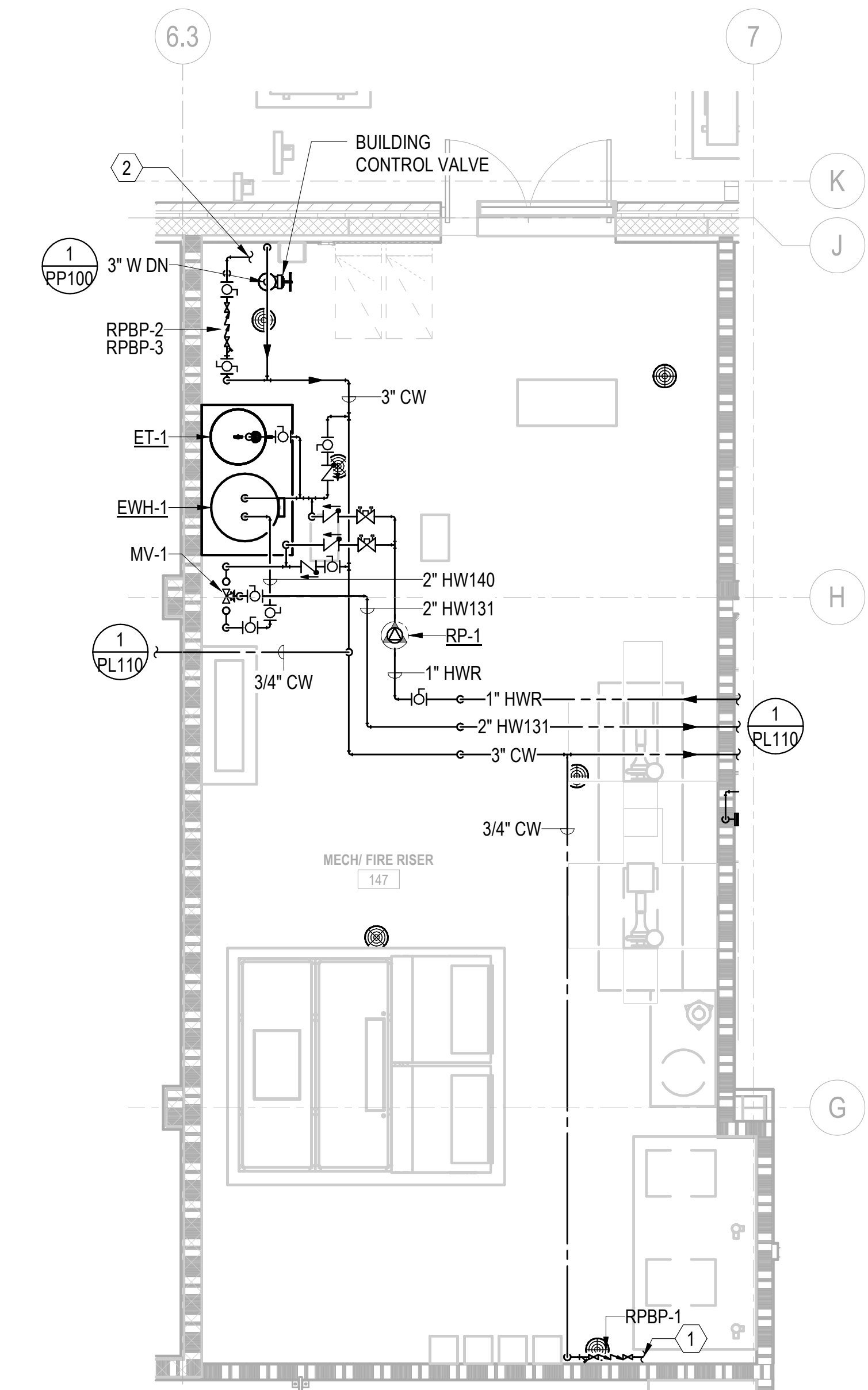
2 ENLARGED PLUMBING PLAN - MECH ROOM - WATER SCALE: 1/4" = 1'-0"
