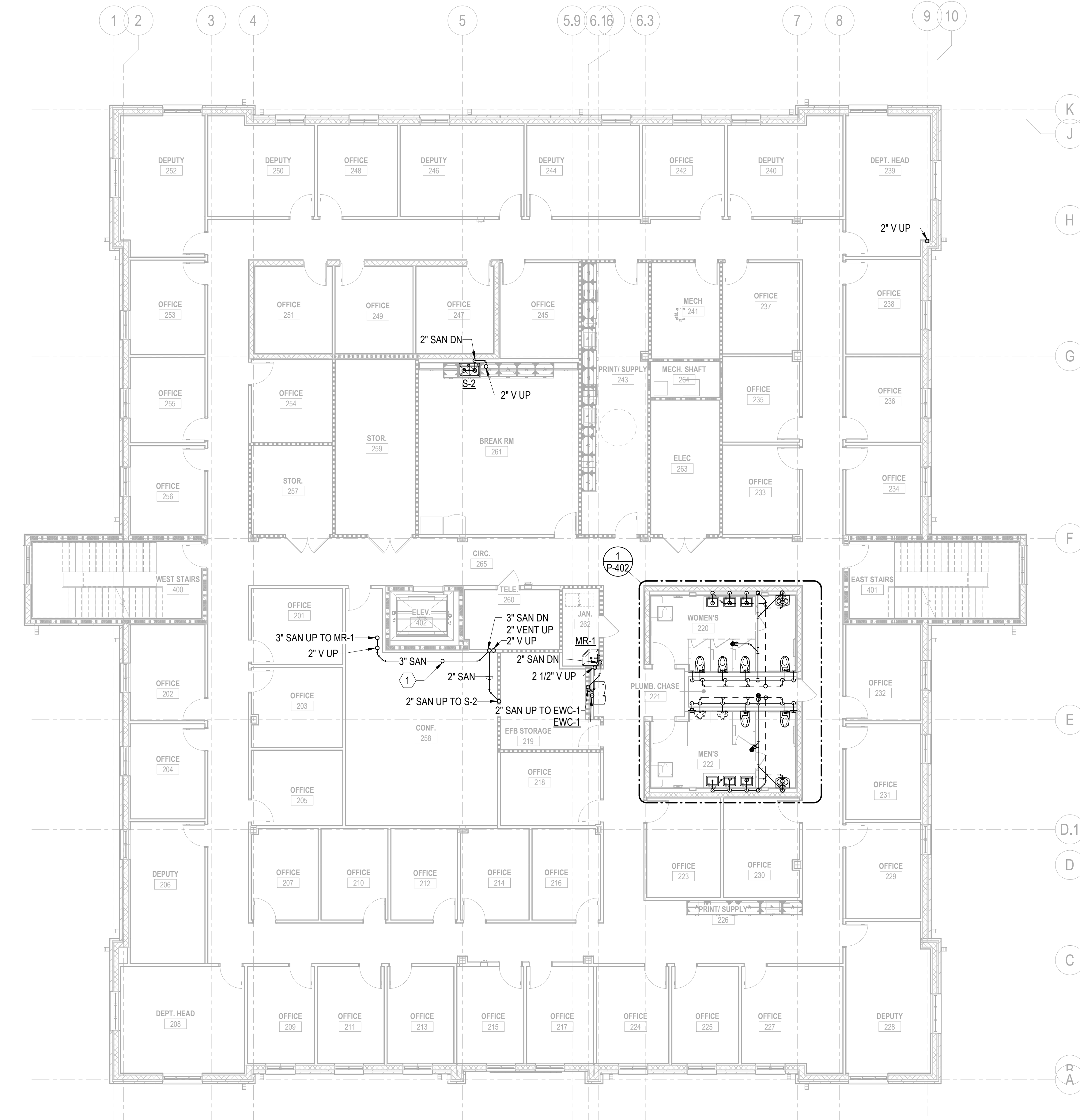
1 PLUMBING - WASTE & VENT - 2ND FLOOR PLAN SCALE: 1/8" = 1'-0"
