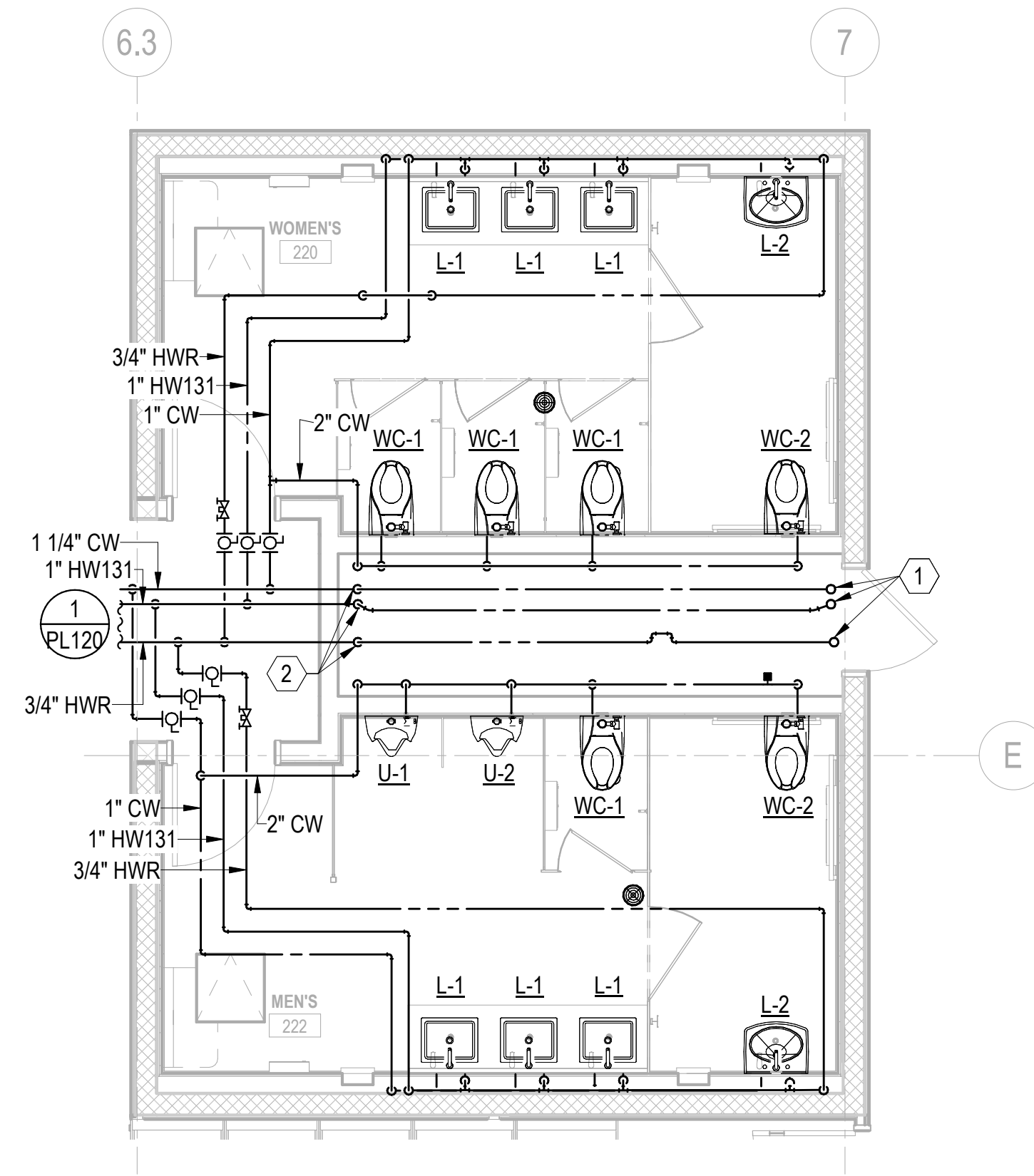
2 ENLARGED PLUMBING PLAN - LEVEL 2 - WATER SCALE: 1/4" = 1'-0"
