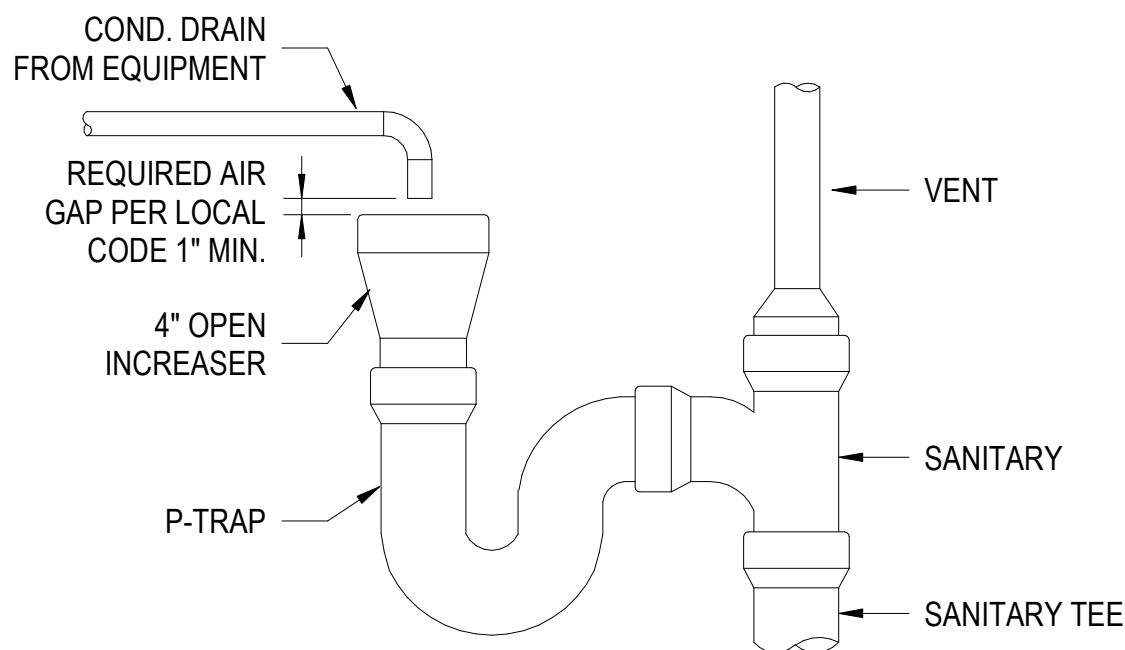
4 TYPICAL AIR GAP DRAIN SCALE:NTS
