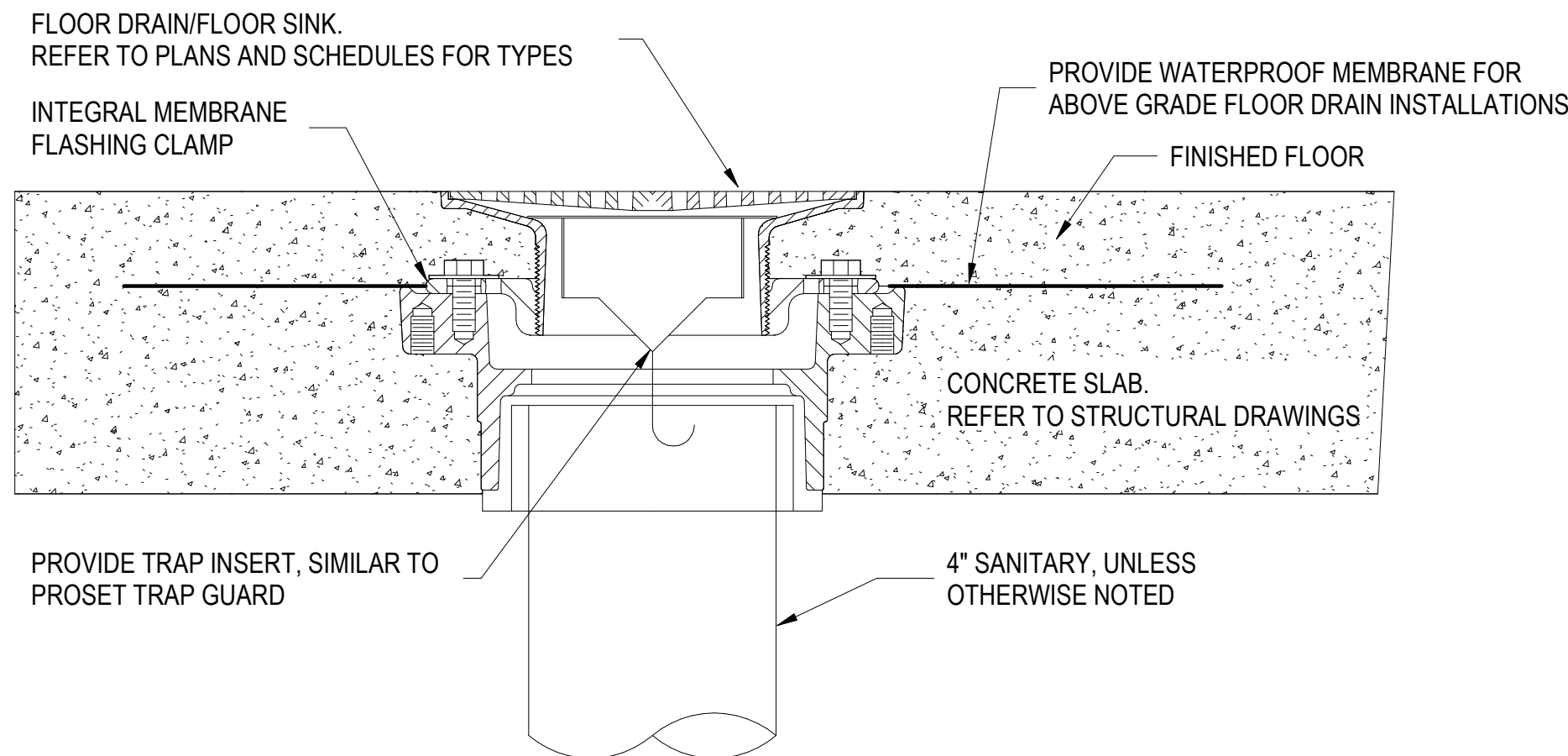
1 FLOOR DRAIN - TRAP SEAL INSERT SCALE:NTS
