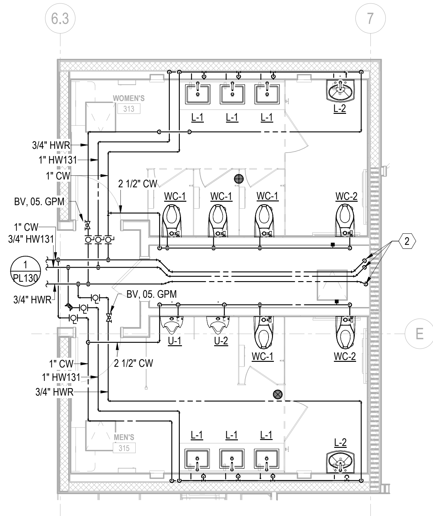
4 ENLARGED PLUMBING PLAN - LEVEL 3 - WATER SCALE: 1/4" = 1'-0"
