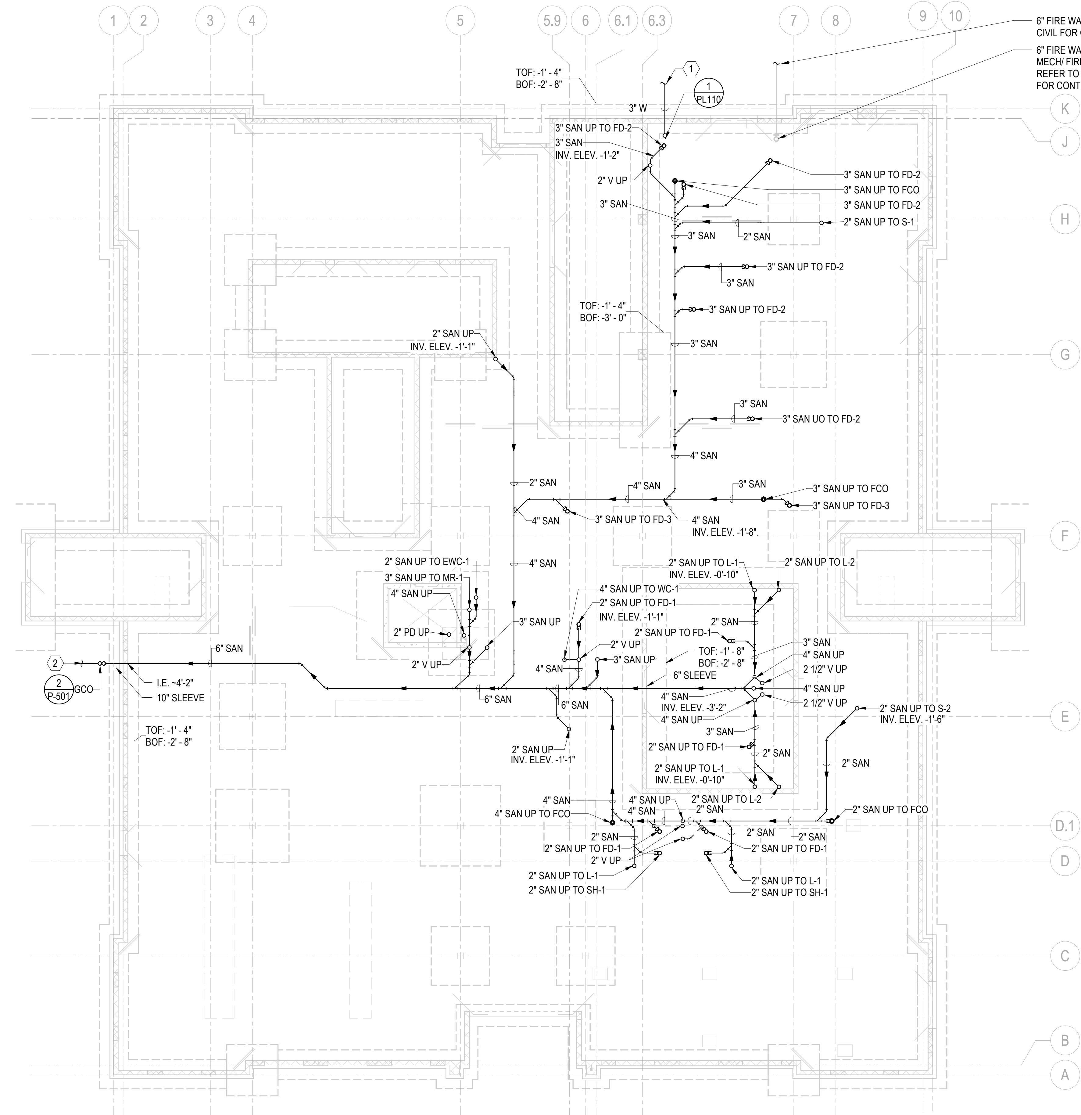
1 PLUMBING - WASTE & VENT - UNDERFLOOR PLAN SCALE: 1/8" = 1'-0"
