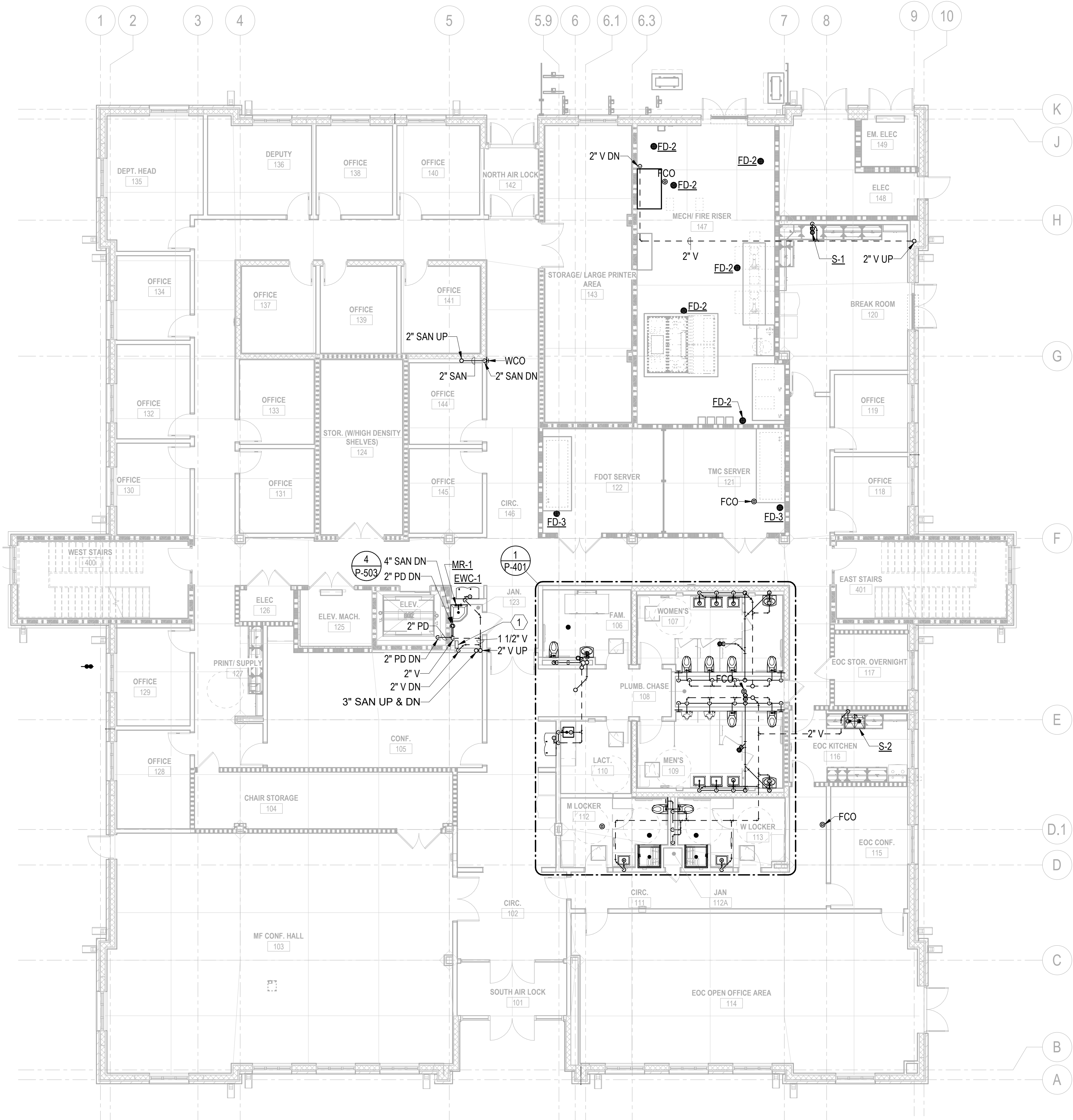
1 PLUMBING - WASTE & VENT - 1ST FLOOR PLAN SCALE: 1/8" = 1'-0"
