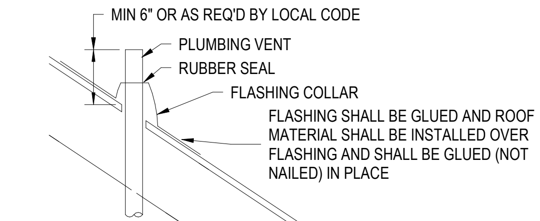
6 VENT THROUGH SLOPED ROOF SCALE:NTS
