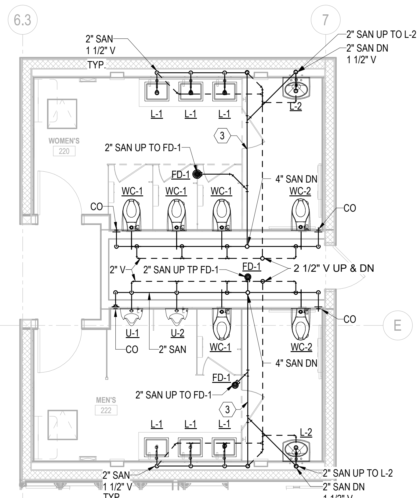
1 ENLARGED PLUMBING PLAN - LEVEL 2 - WASTE & VENT SCALE: 1/4" = 1'-0"
