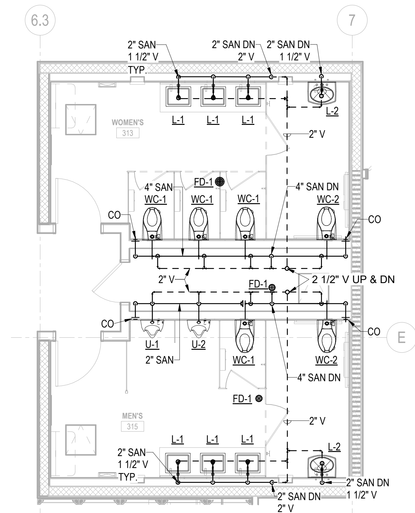
3 ENLARGED PLUMBING PLAN - LEVEL 3 - WASTE & VENT SCALE: 1/4" = 1'-0"
