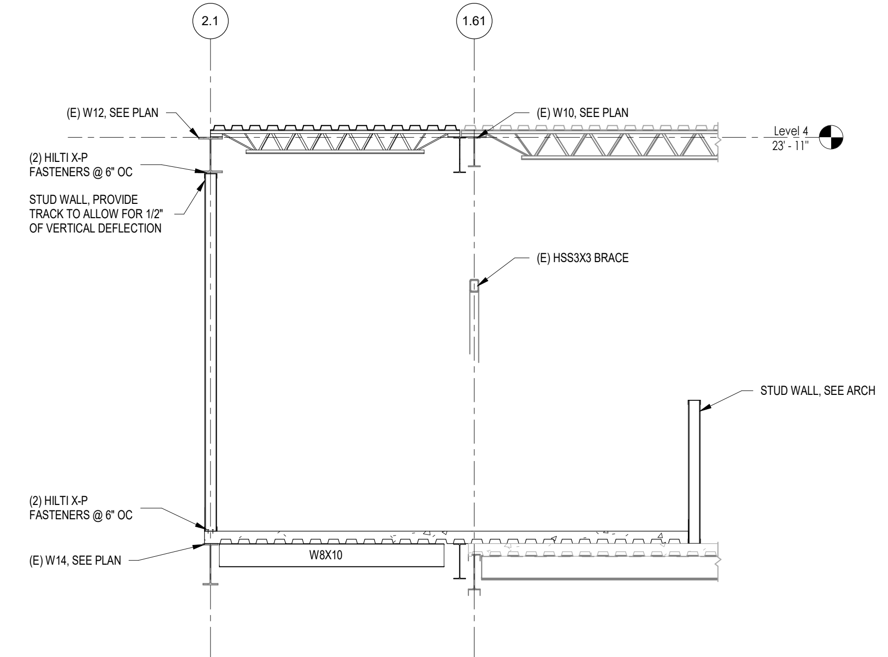
5 Overbuild Section S201 SCALE: 3/8" = 1'-0"
