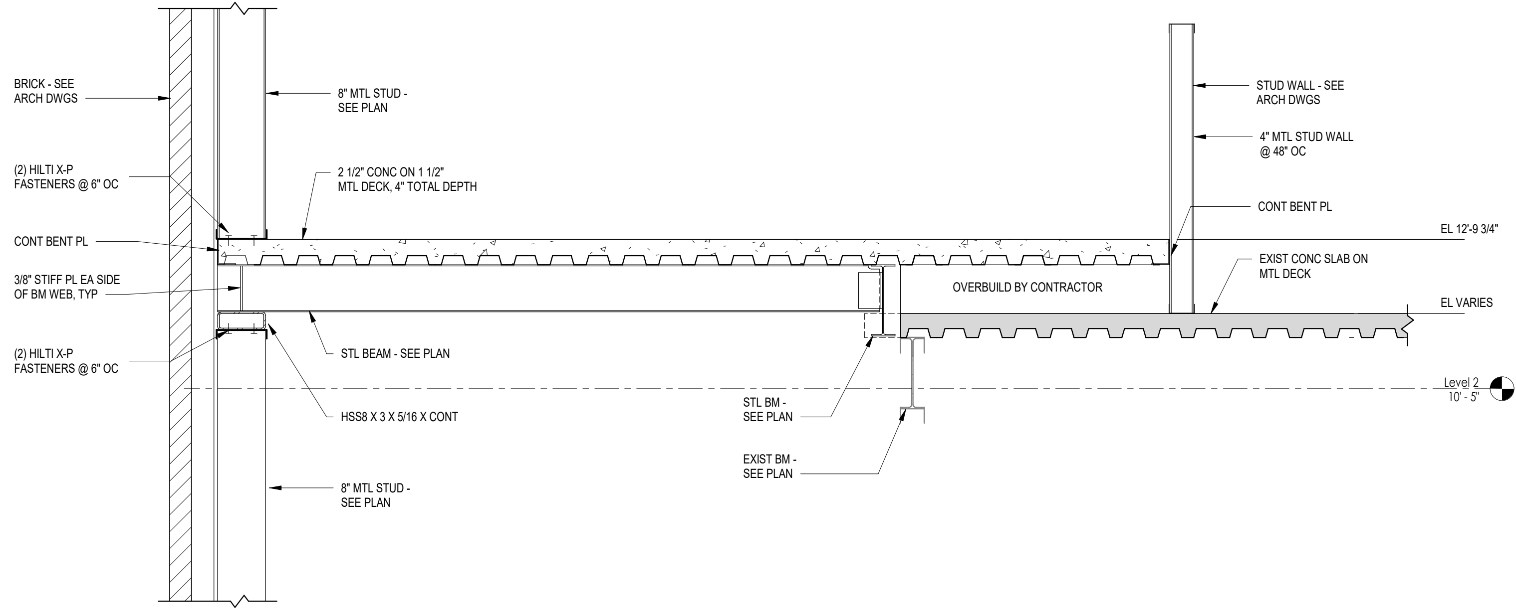
1 Section at Second Flr S201 SCALE: 3/4" = 1'-0"
