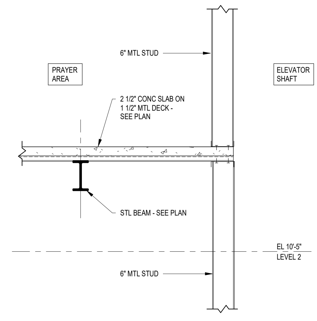
2 Section at Elevator S201 SCALE: 3/4" = 1'-0"
