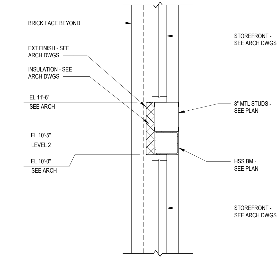
3 Storefront Section at Level 2 S201 SCALE: 3/4" = 1'-0"
