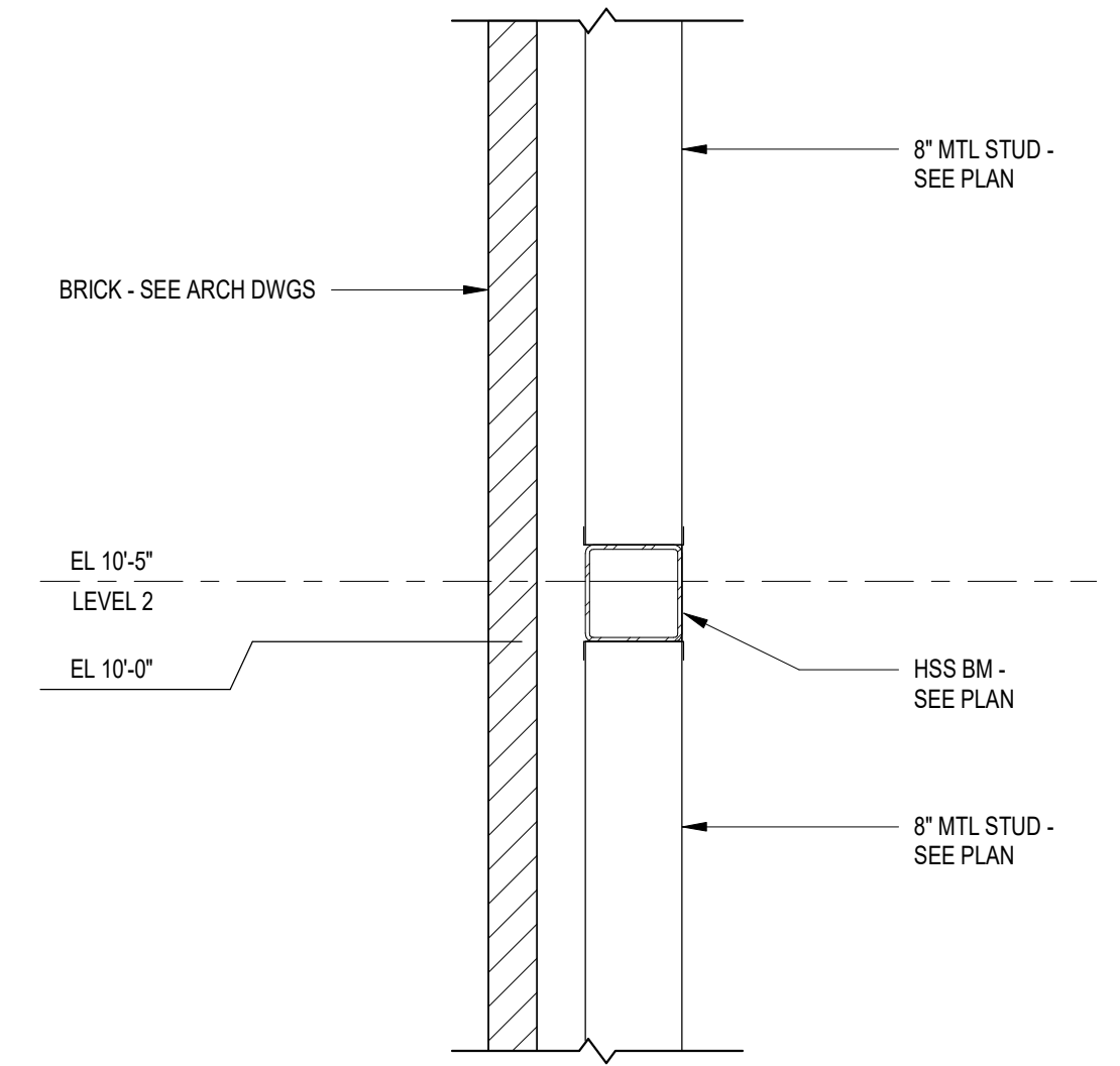
4 Beam at Level 2 Ext Wall S201 SCALE: 3/4" = 1'-0"
