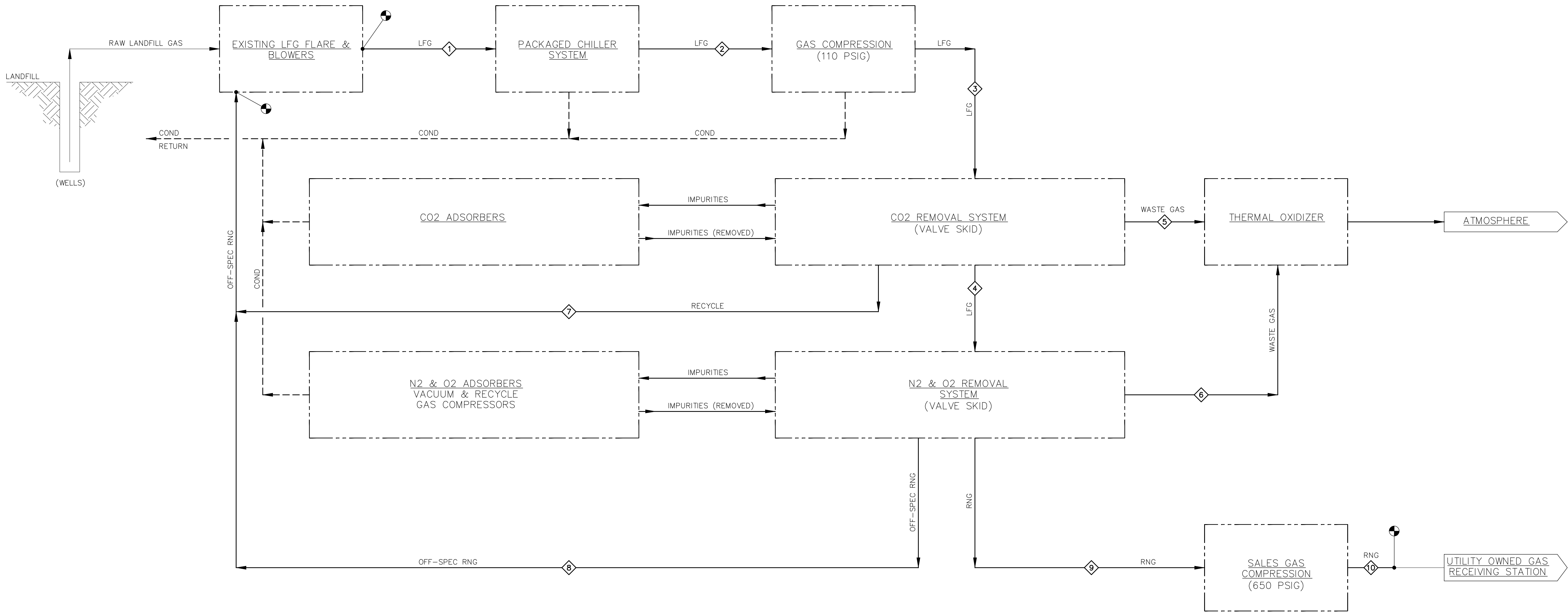
COFFEE COUNTY LANDFILL HIGH BTU PROCESS FLOW DIAGRAM
