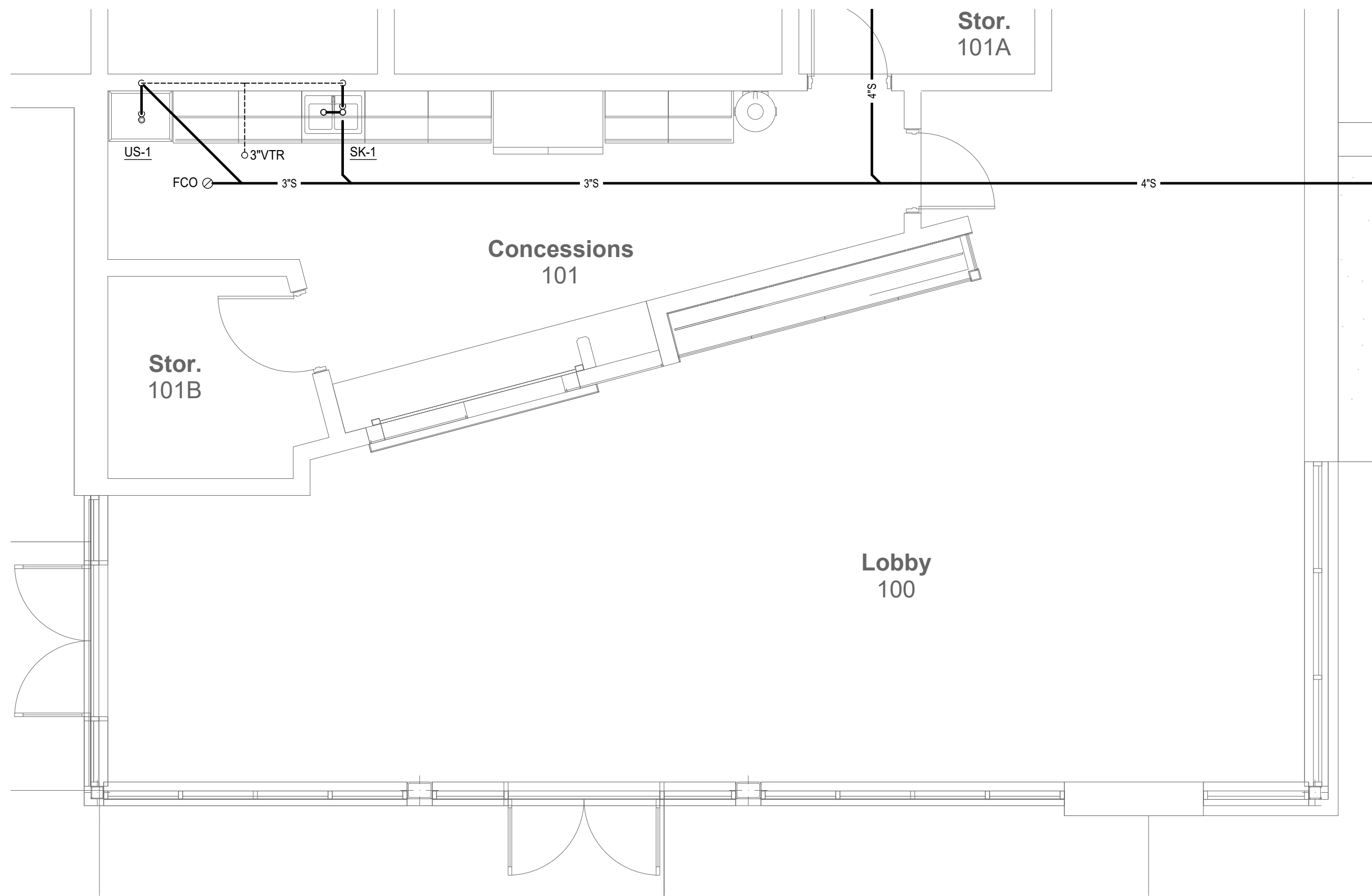
3 Plumbing Enlarged Plan - Sanitary 1/4" = 1'-0"
