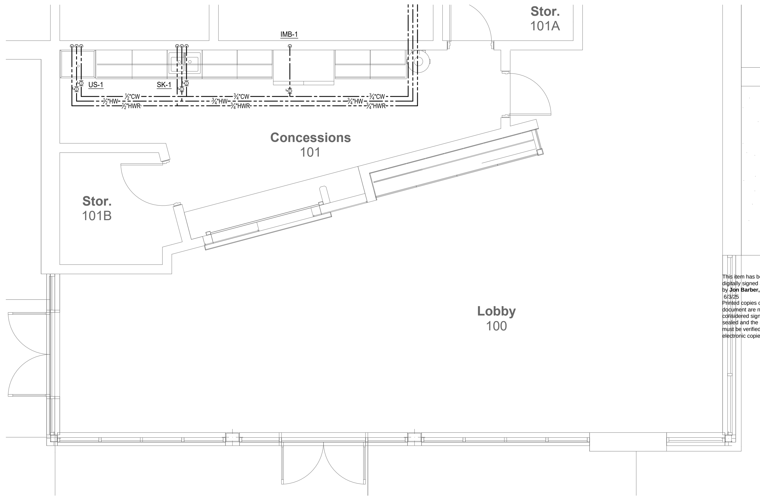
4 Plumbing Enlarged Plan - Domestic Water 1/4" = 1'-0"
