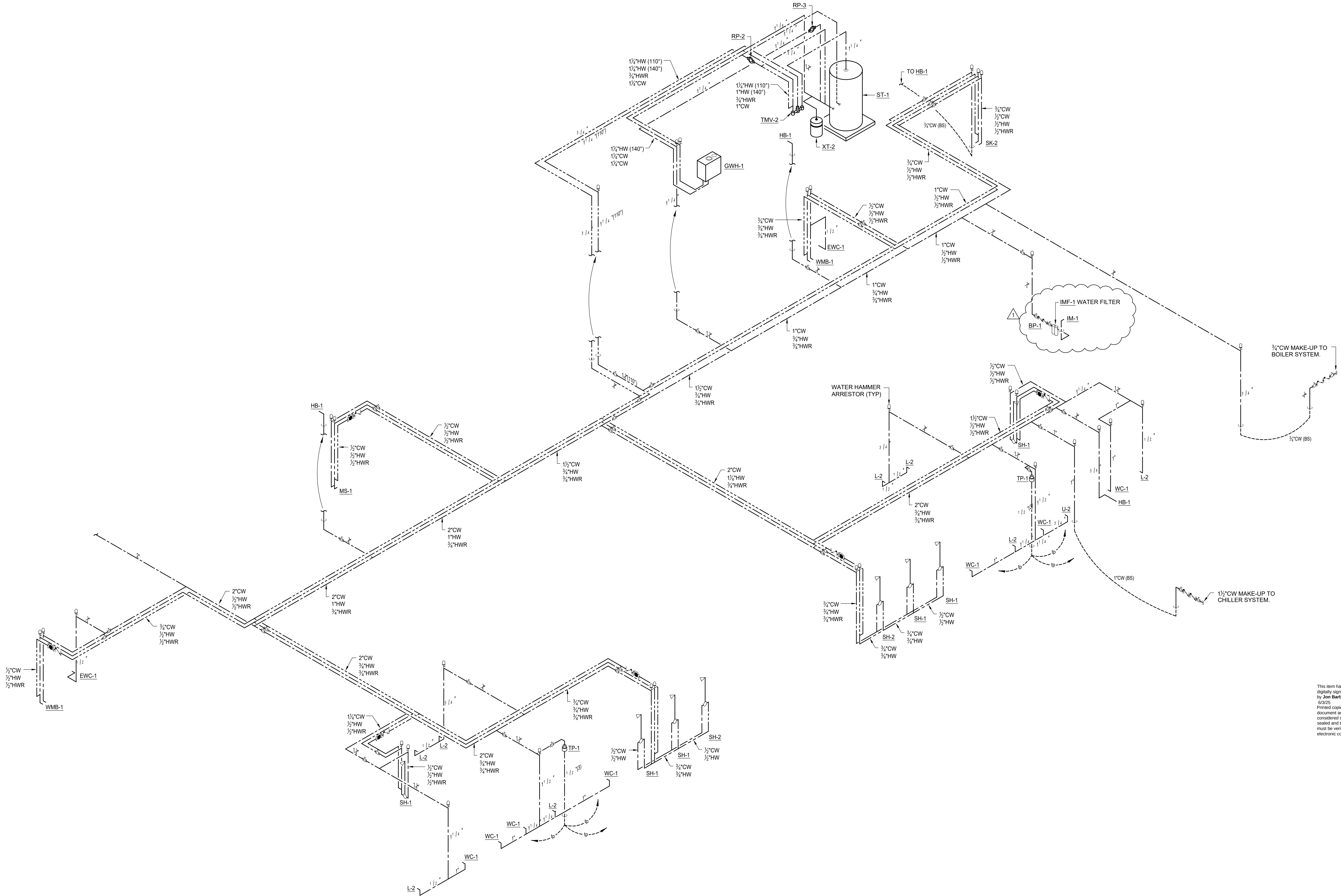
1 Plumbing Riser - Domestic Water NTS
