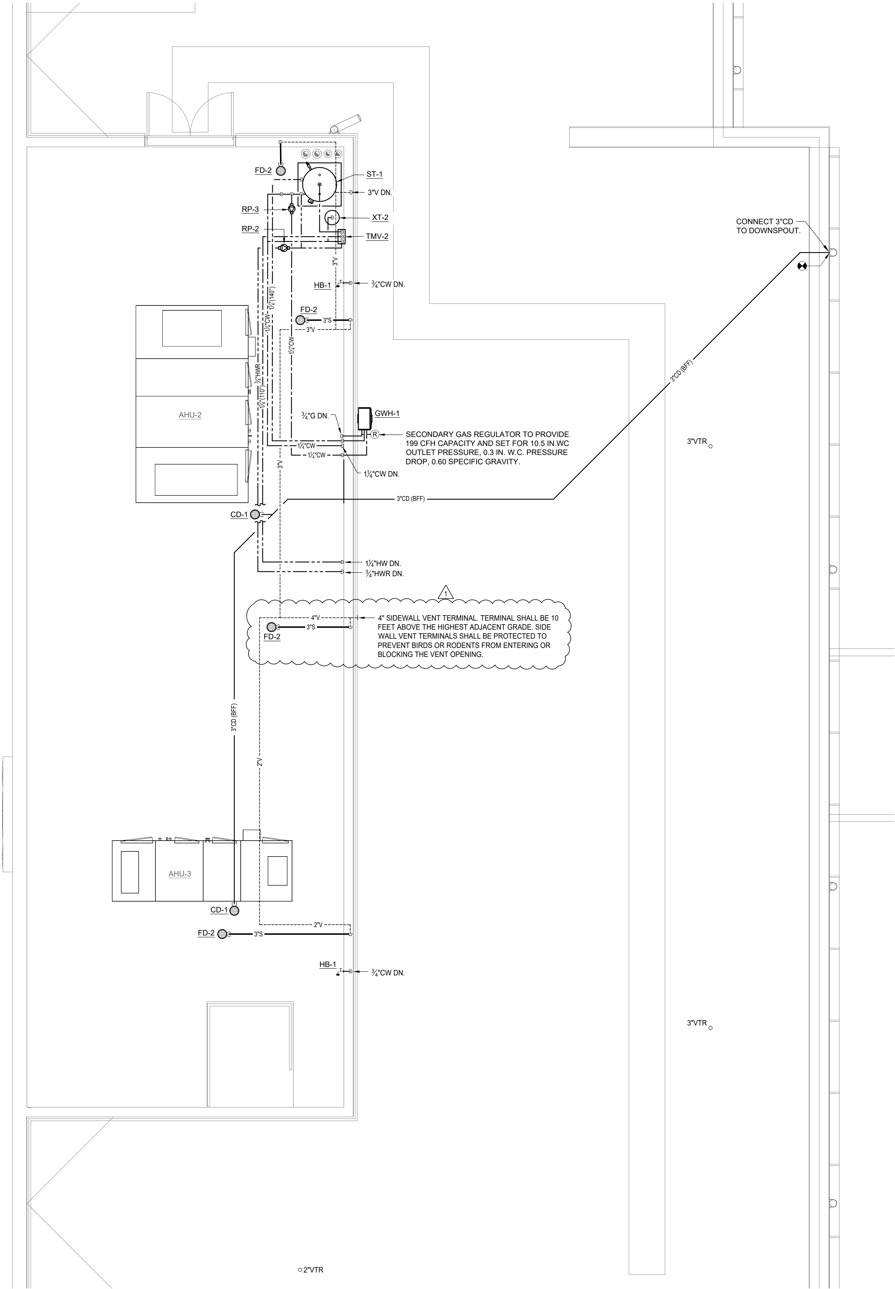
1 Plumbing Enlarged Plan - Equipment Platform
