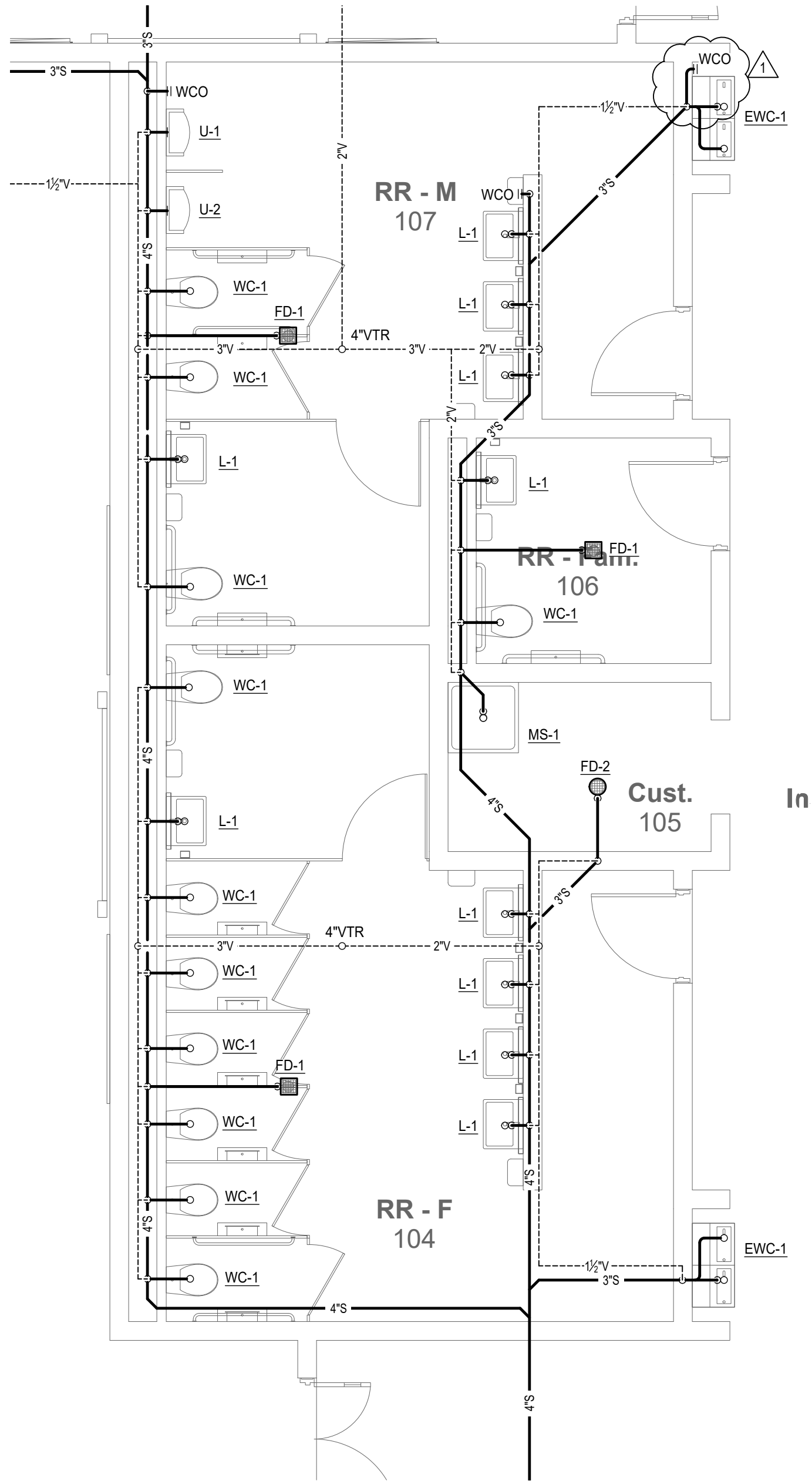
1 Plumbing Enlarged Plan - Sanitary 1/4" = 1'-0"
