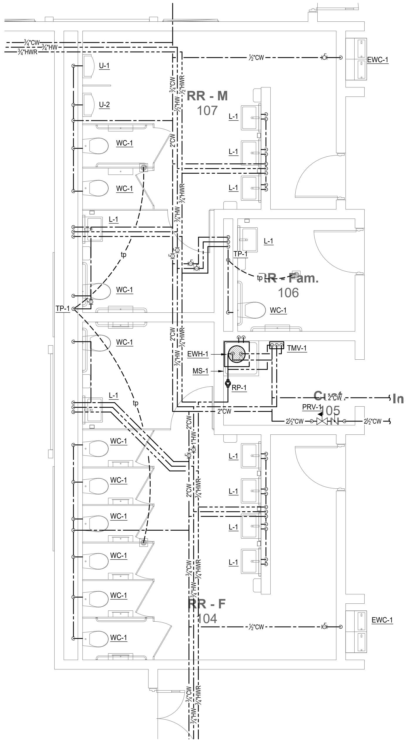
2 Plumbing Enlarged Plan - Domestic Water 1/4" = 1'-0"
