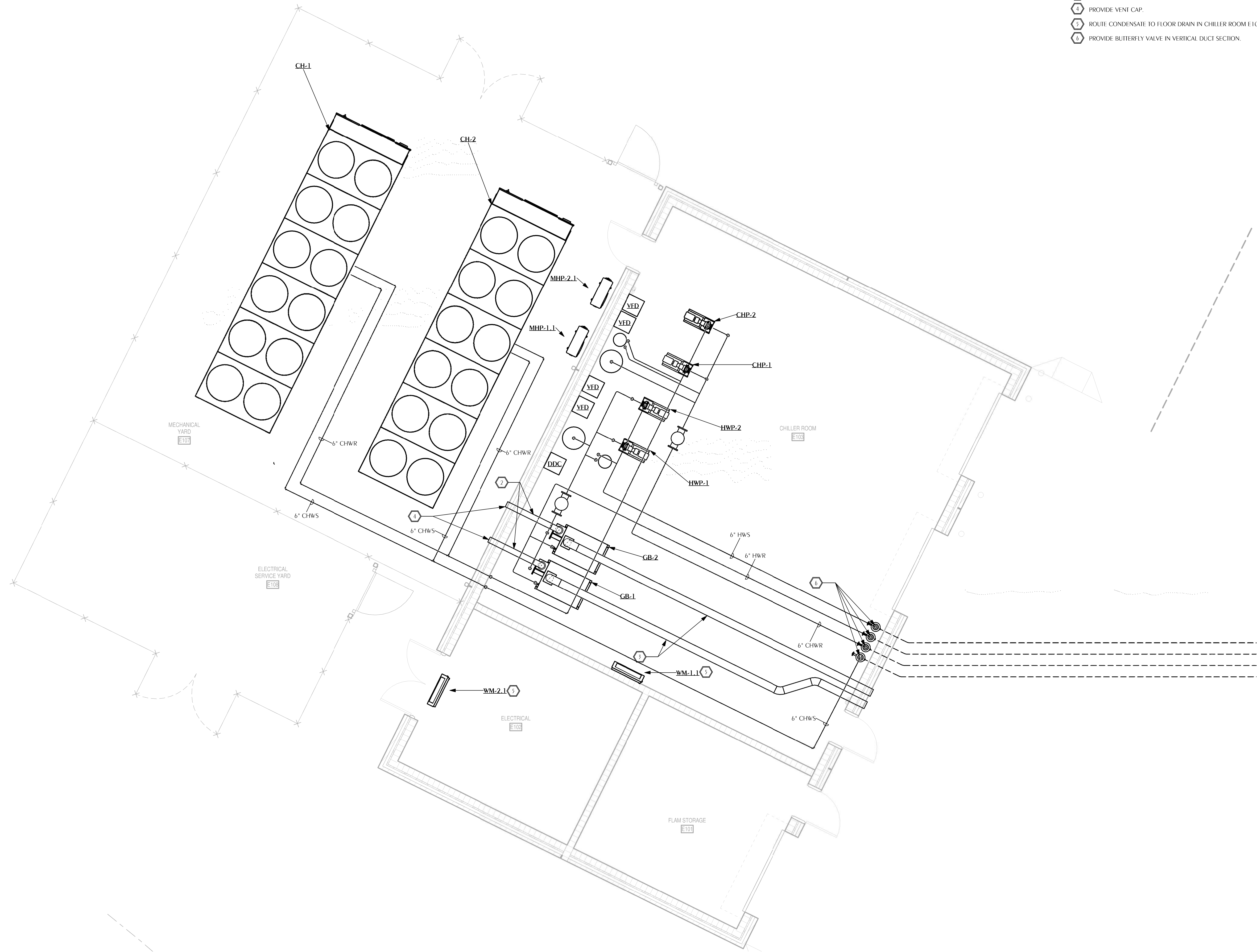
1 HVAC CENTRAL PLANT PLAN MS-111 SCALE: 1/4" = 1'-0" PROJECT NORTH TRUE NORTH
